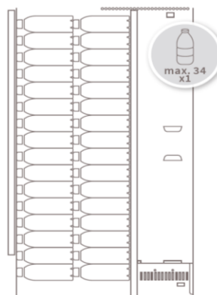
Side section column with bottles
